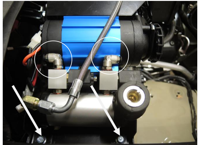
Mount manifold to bracket if applicable - note orientation of manifold brackets (do not tighten). ARB Locker Solenoids installed to show orientations (Step 1B)
