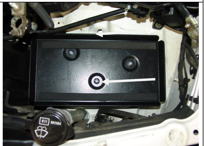
Install Adhesive Pads ( Step 4A )
